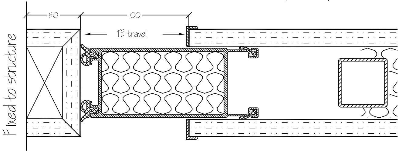
PLAN SECTION at PANEL JOINT
